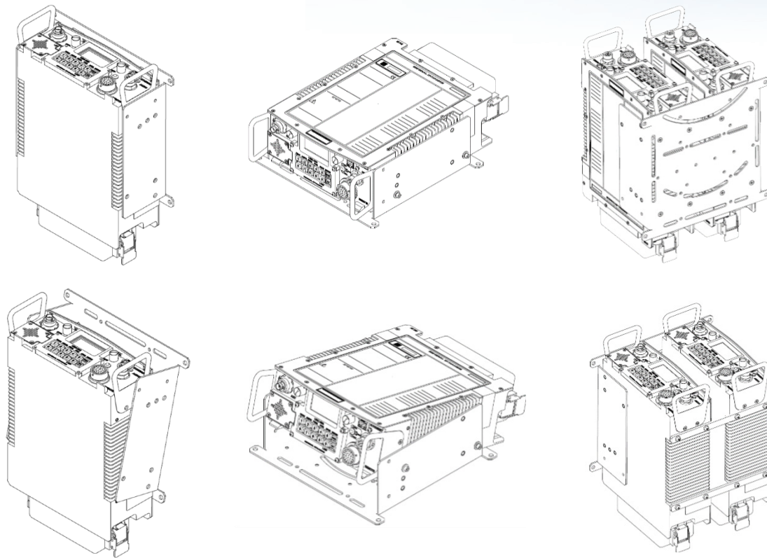
SINGLE AND DUAL RADIO AND BRACKET MOUNTING
