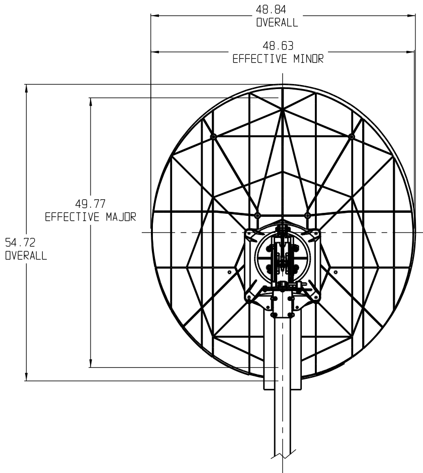
GEOMETRY, 2120 SERIES ANTENNA
