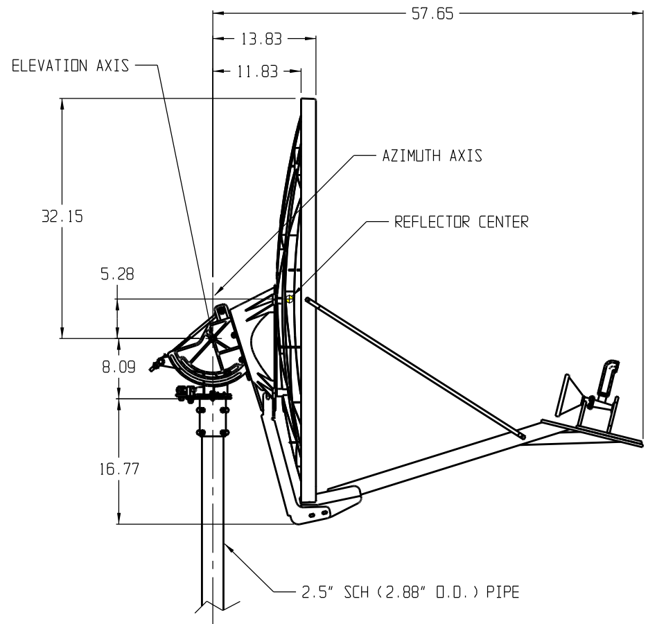
GEOMETRY, 2120 SERIES ANTENNA
